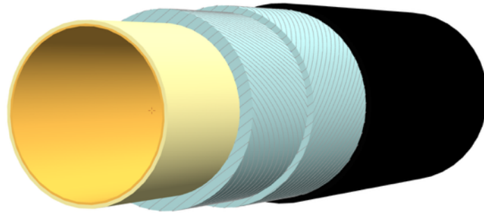
3D diagram of POE/HDPE/GFT/HDPE pipe
