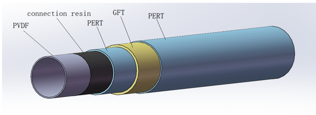
3D diagram and physical product illustration of PVDF/bonding
